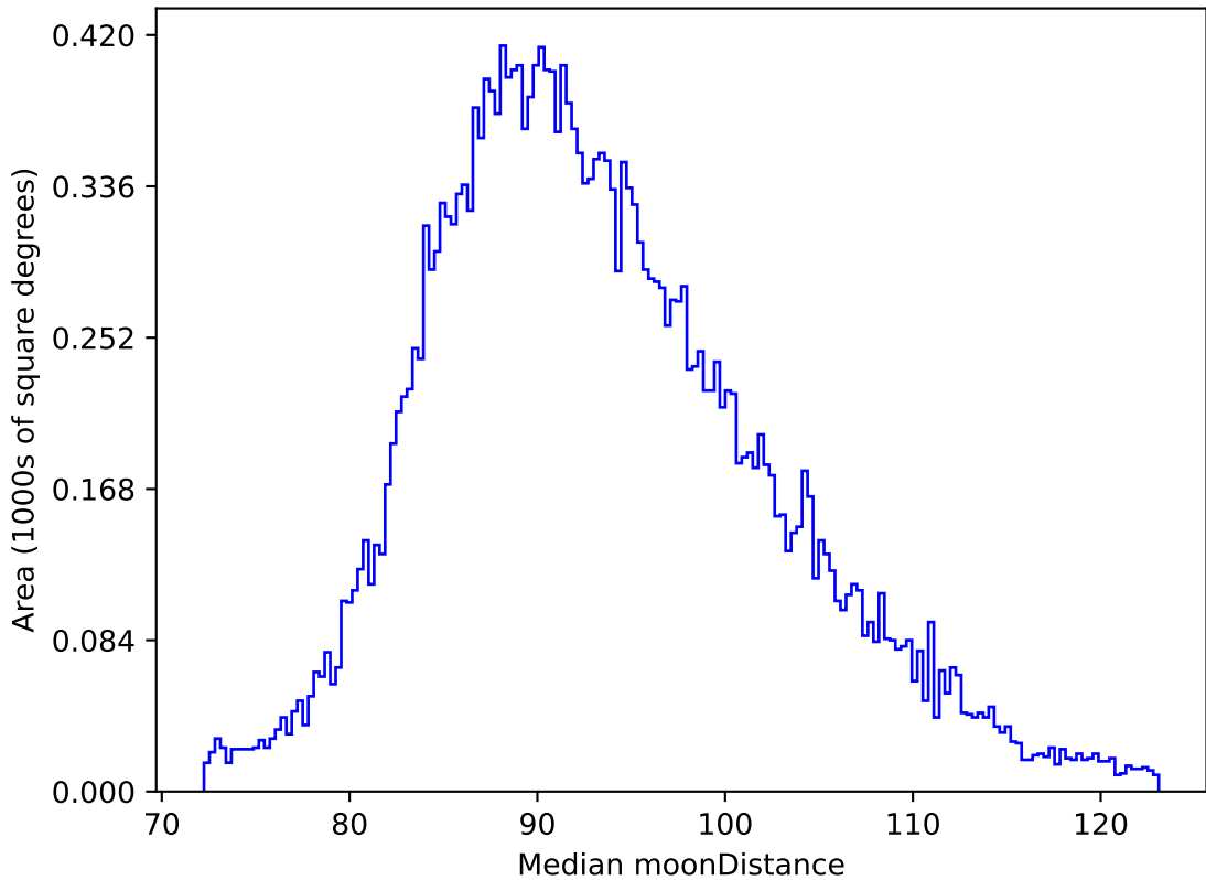
too_elab_r128_d2_gz_v3.4_10yrs All sky i band: Median moonDistance
