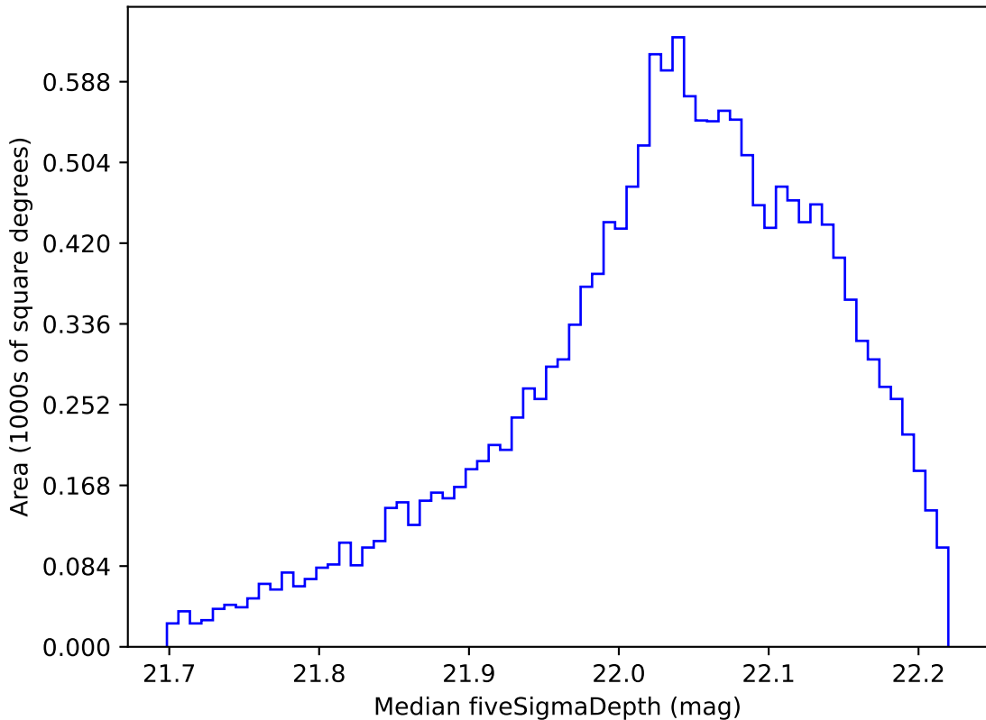
too_elab_r128_d2_gz_v3.4_10yrs WFD y band: Median fiveSigmaDepth
