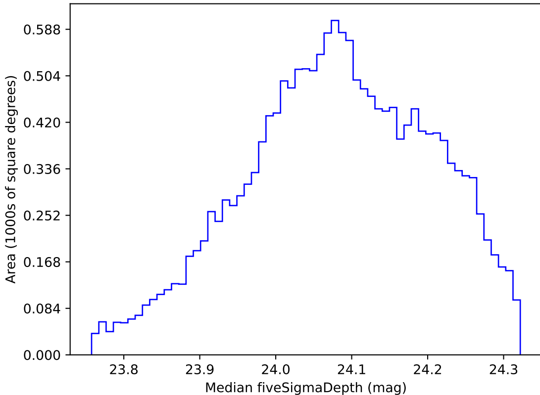
too_elab_r128_d2_gz_v3.4_10yrs WFD r band: Median fiveSigmaDepth
