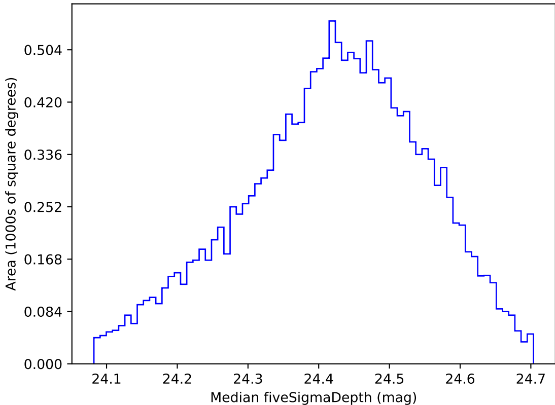
too_elab_r128_d2_gz_v3.4_10yrs WFD g band: Median fiveSigmaDepth
