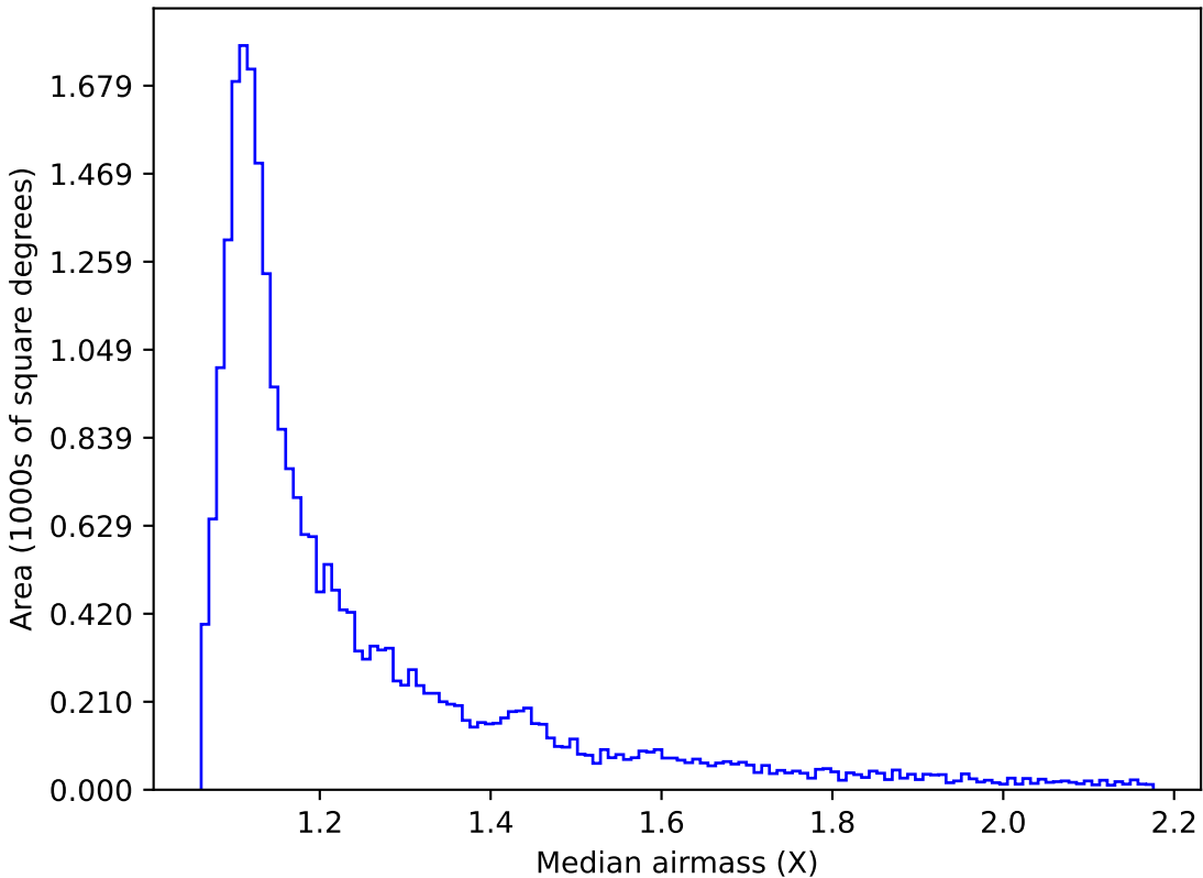
too_elab_r128_d2_gz_v3.4_10yrs Yr 1 z band: Median airmass
