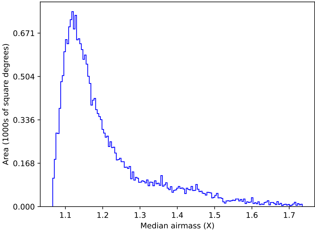
too_elab_r128_d2_gz_v3.4_10yrs Yr 1 y band: Median airmass
