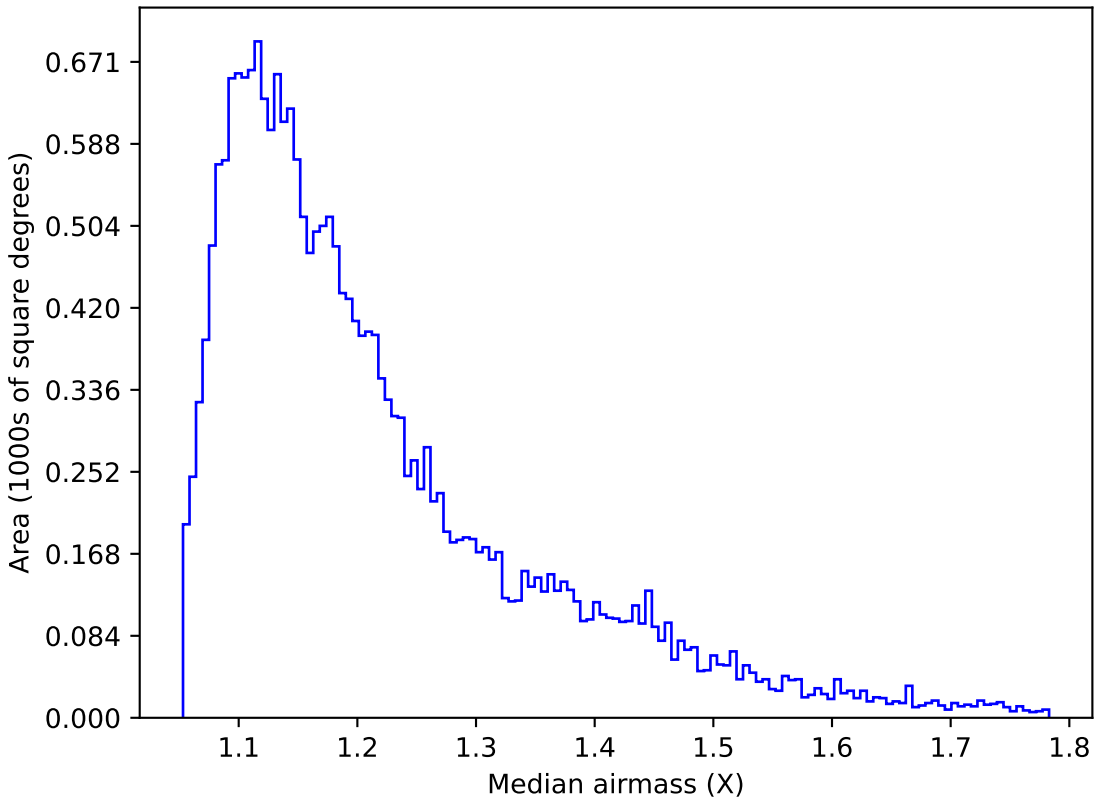
too_elab_r128_d2_gz_v3.4_10yrs Yr 1 u band: Median airmass
