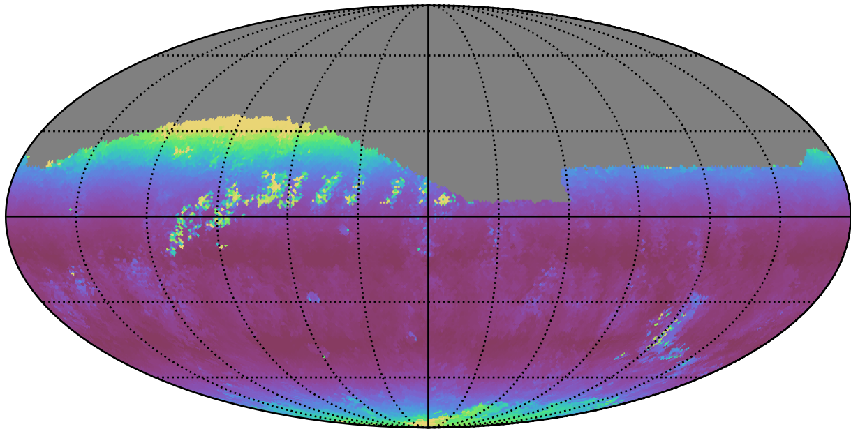
too_elab_r128_d2_gz_v3.4_10yrs Yr 1 r band: Median airmass
