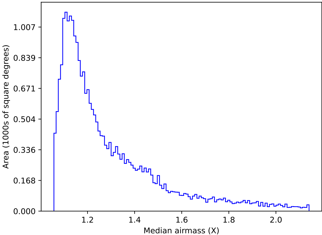
too_elab_r128_d2_gz_v3.4_10yrs Yr 1 g band: Median airmass
