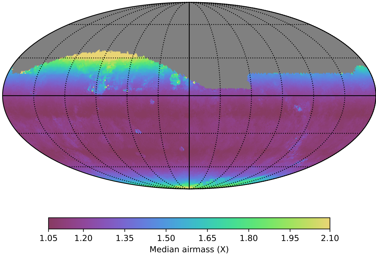
too_elab_r128_d2_gz_v3.4_10yrs Yr 1 all bands: Median airmass
