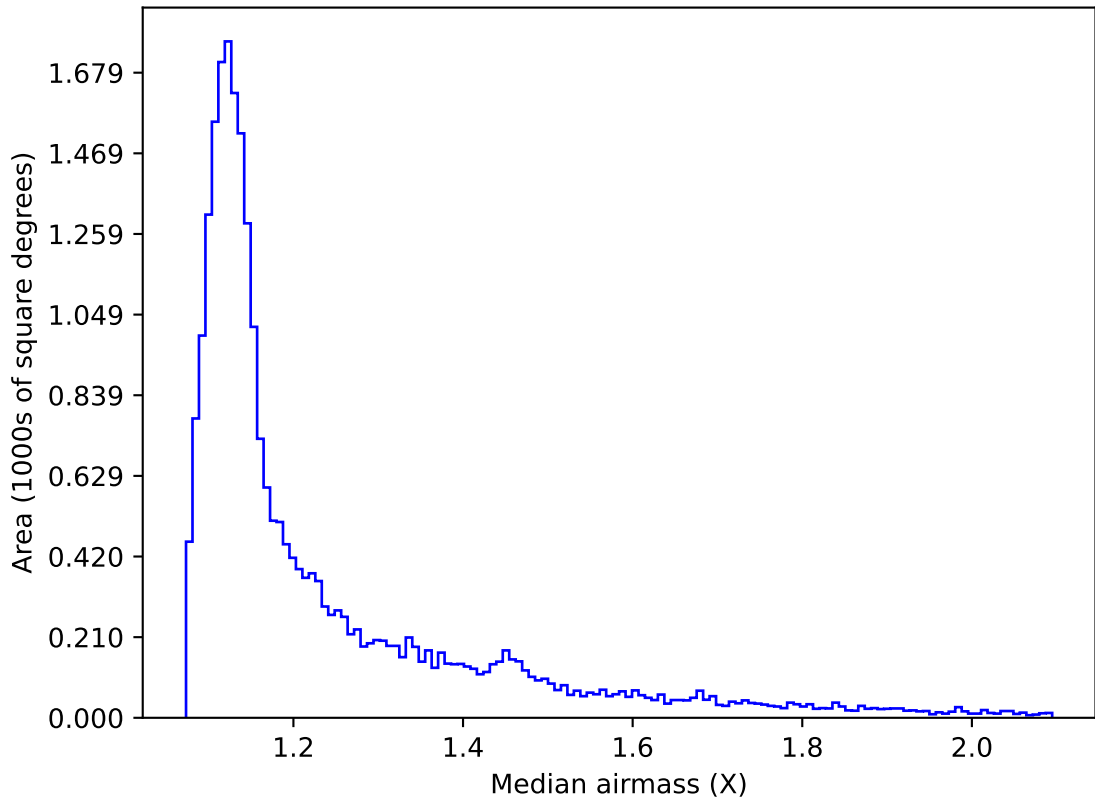
too_elab_r128_d2_gz_v3.4_10yrs Yr 1 all bands: Median airmass
