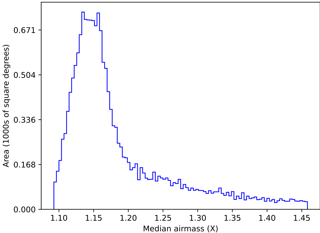
too_elab_r128_d2_gz_v3.4_10yrs WFD z band: Median airmass
