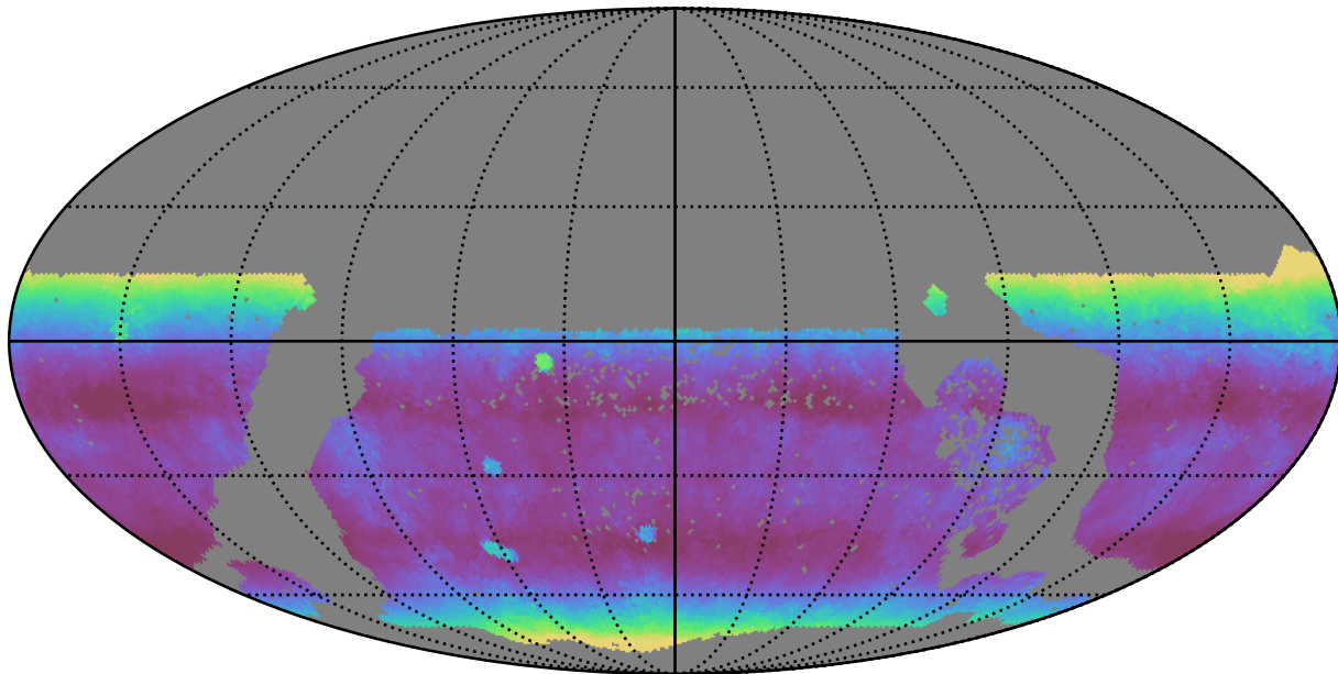
too_elab_r128_d2_gz_v3.4_10yrs WFD y band: Median airmass
