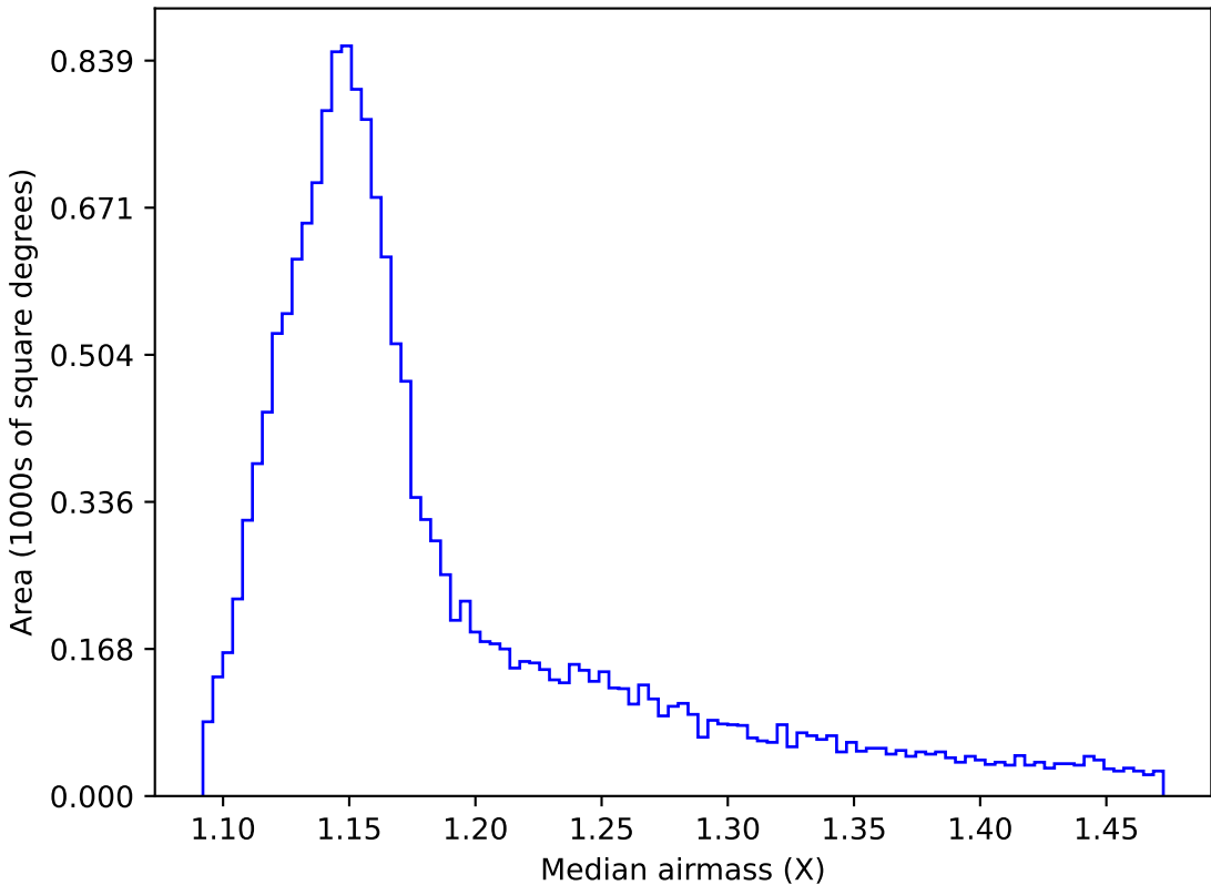
too_elab_r128_d2_gz_v3.4_10yrs WFD y band: Median airmass
