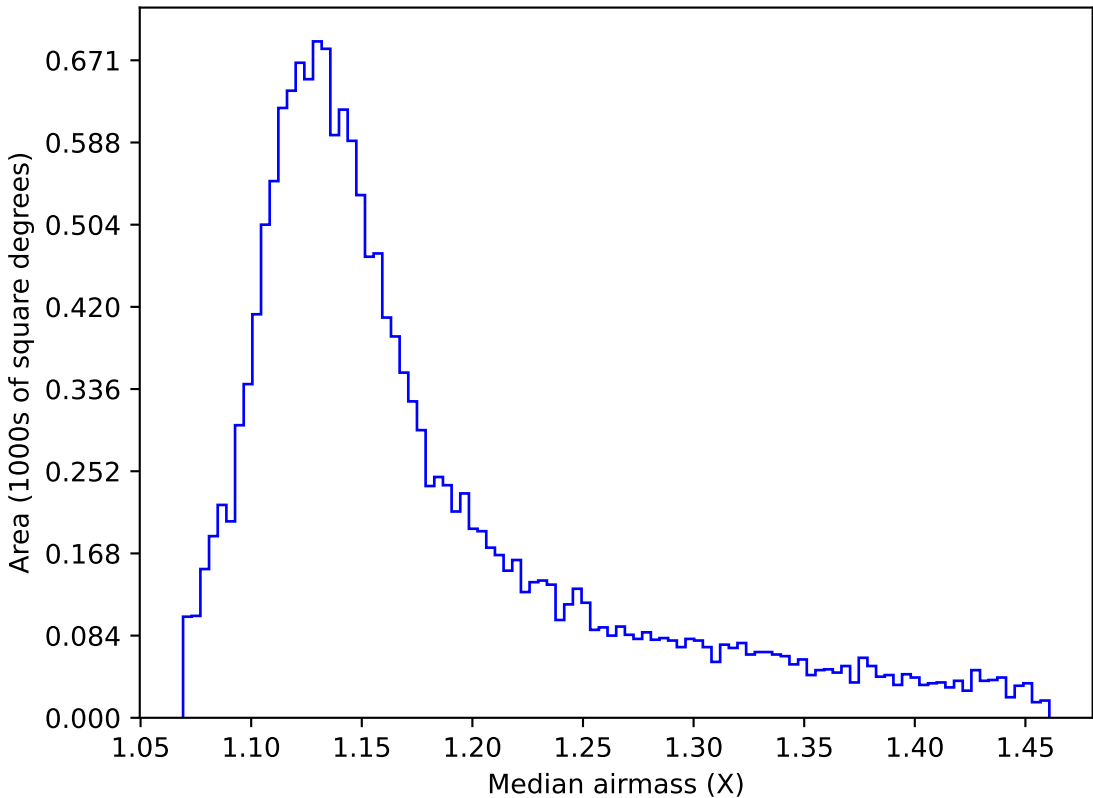
too_elab_r128_d2_gz_v3.4_10yrs WFD u band: Median airmass
