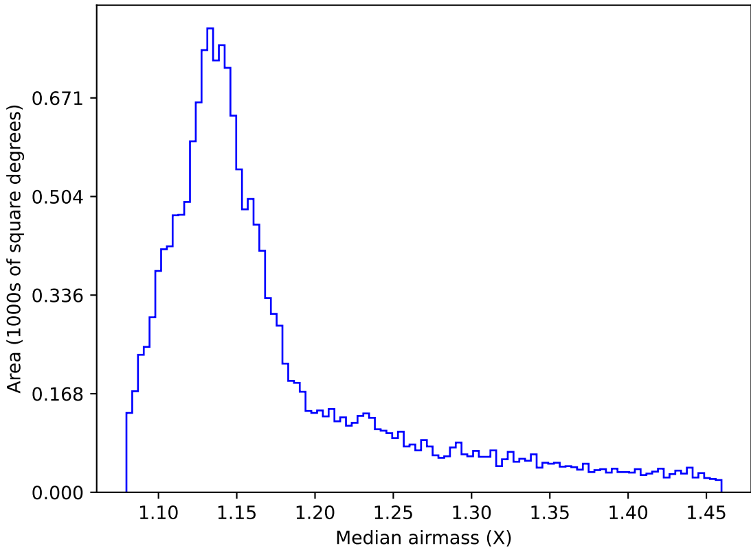
too_elab_r128_d2_gz_v3.4_10yrs WFD i band: Median airmass
