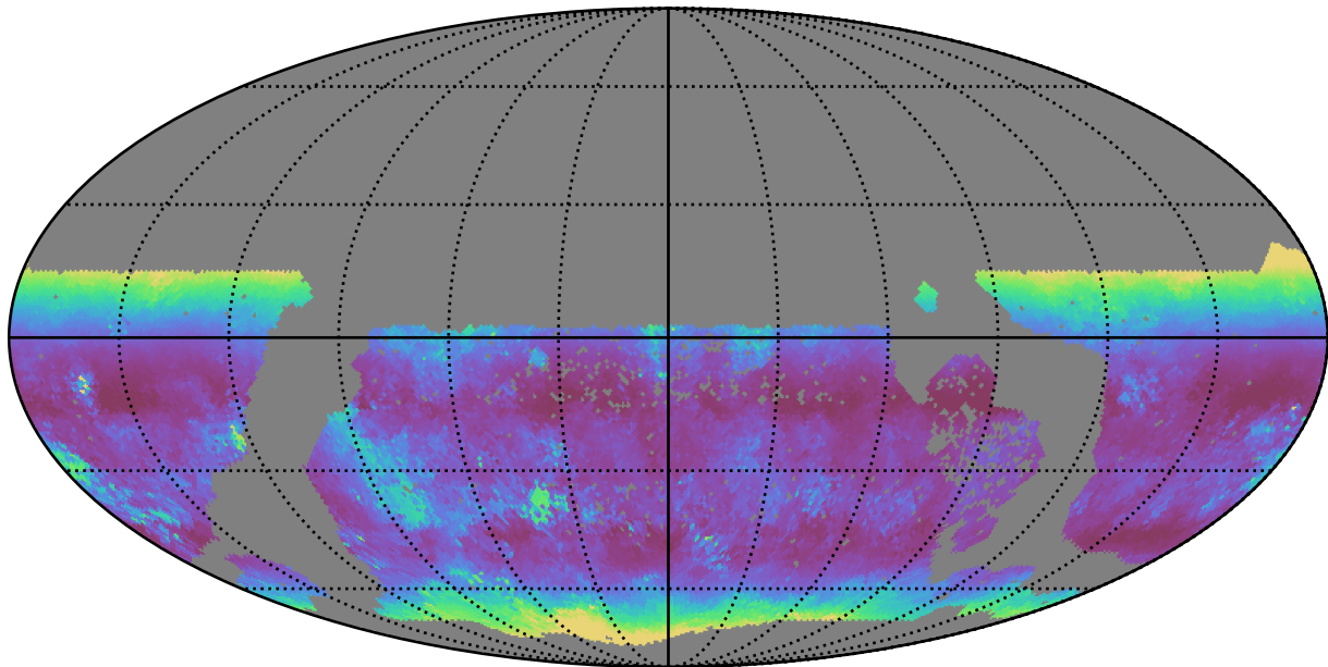
too_elab_r128_d2_gz_v3.4_10yrs WFD g band: Median airmass
