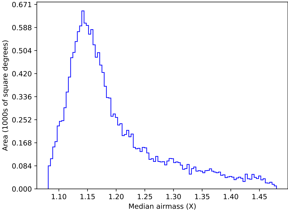
too_elab_r128_d2_gz_v3.4_10yrs WFD g band: Median airmass
