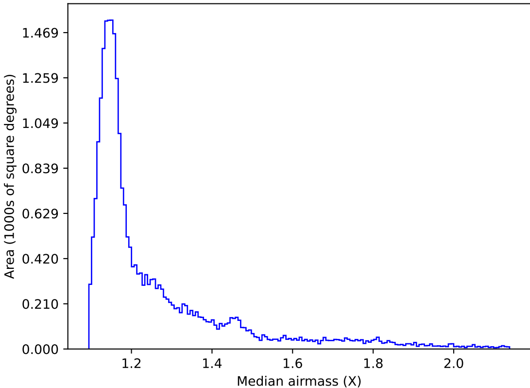
too_elab_r128_d2_gz_v3.4_10yrs All sky z band: Median airmass
