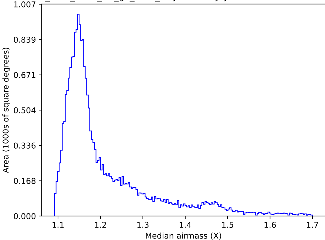
too_elab_r128_d2_gz_v3.4_10yrs All sky y band: Median airmass
