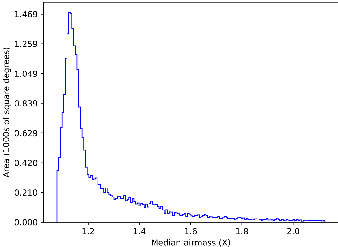
too_elab_r128_d2_gz_v3.4_10yrs All sky r band: Median airmass
