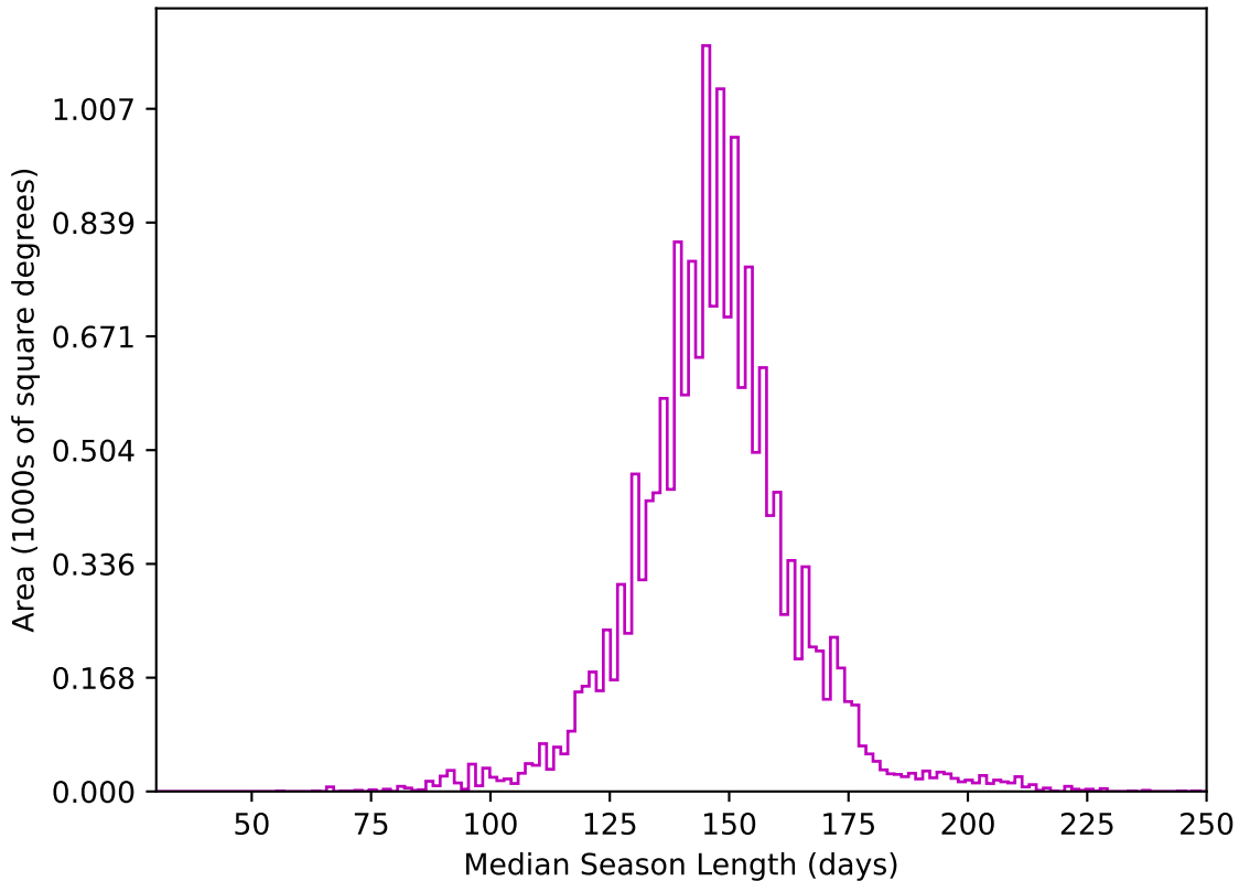
too_elab_r128_d2_gz_v3.4_10yrs WFD z band: Median Season Length
