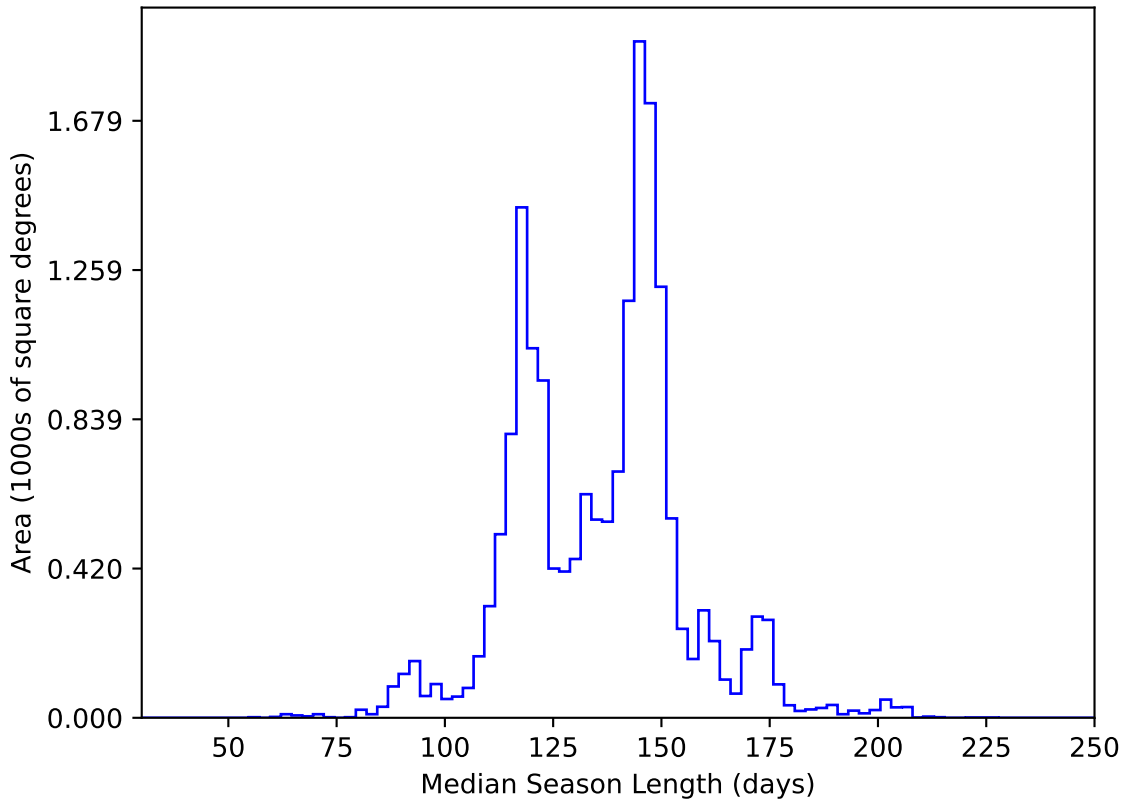
too_elab_r128_d2_gz_v3.4_10yrs WFD y band: Median Season Length
