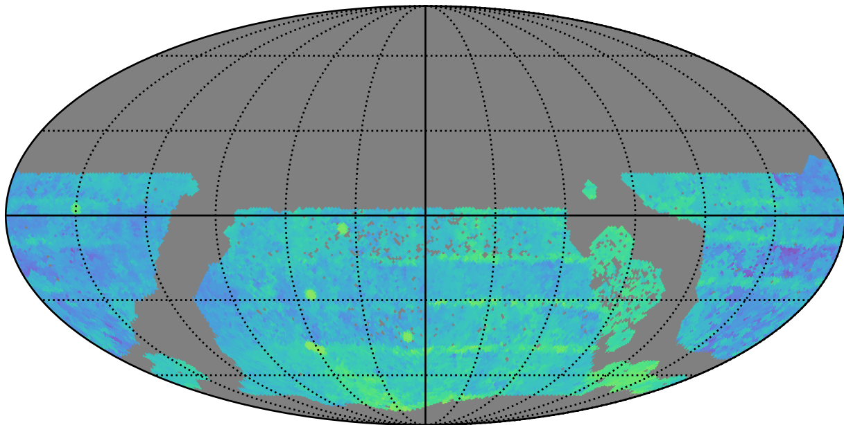
too_elab_r128_d2_gz_v3.4_10yrs WFD r band: Median Season Length
