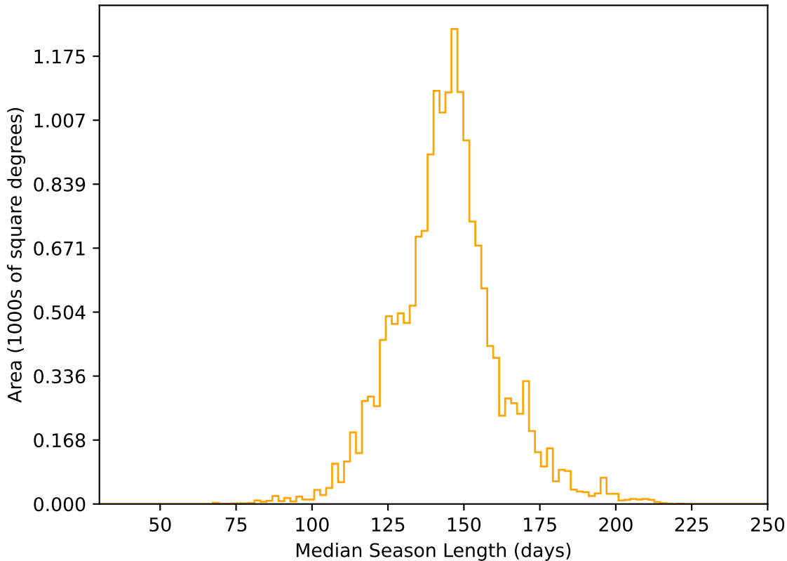
too_elab_r128_d2_gz_v3.4_10yrs WFD r band: Median Season Length
