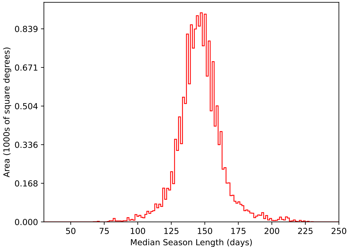
too_elab_r128_d2_gz_v3.4_10yrs WFD i band: Median Season Length
