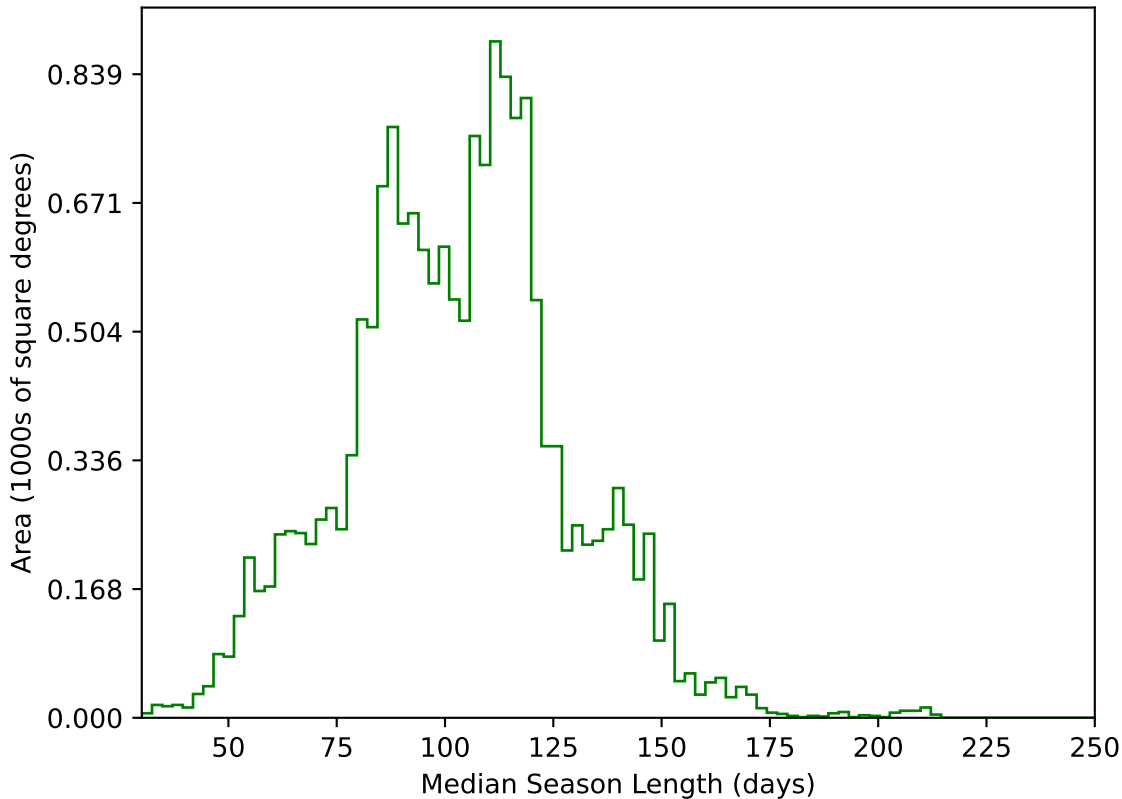
too_elab_r128_d2_gz_v3.4_10yrs WFD g band: Median Season Length
