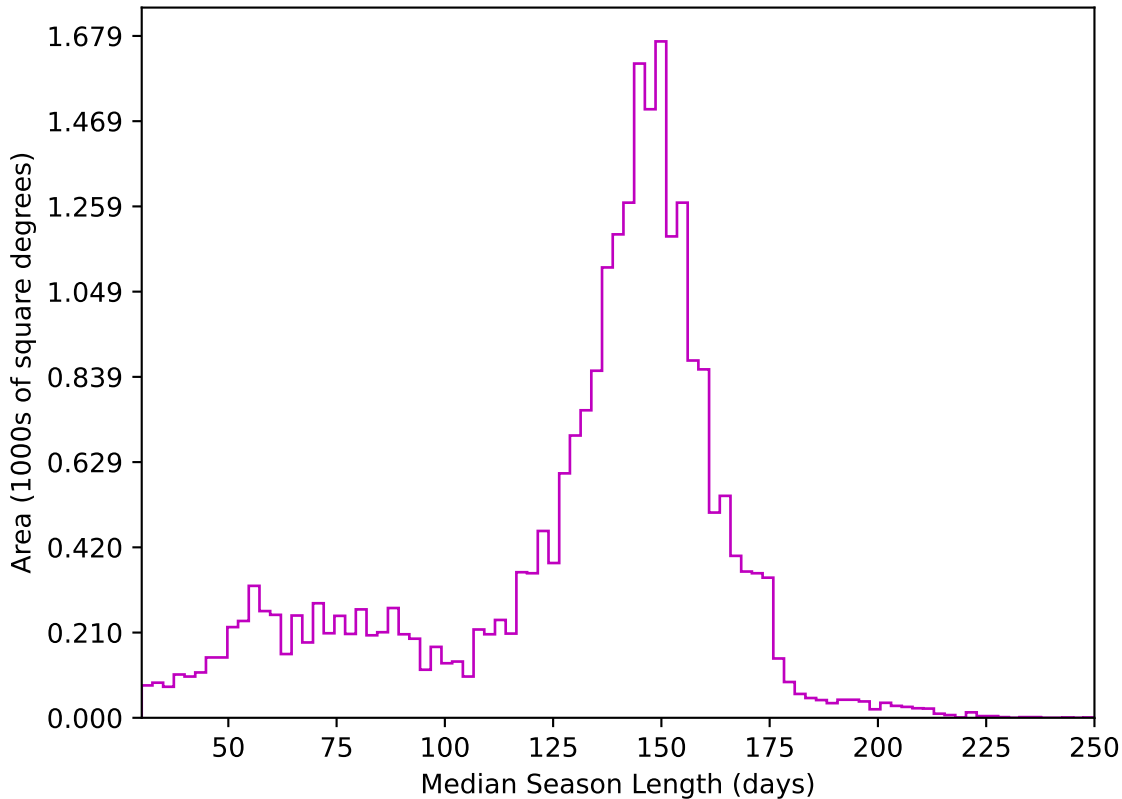
too_elab_r128_d2_gz_v3.4_10yrs All sky z band: Median Season Length
