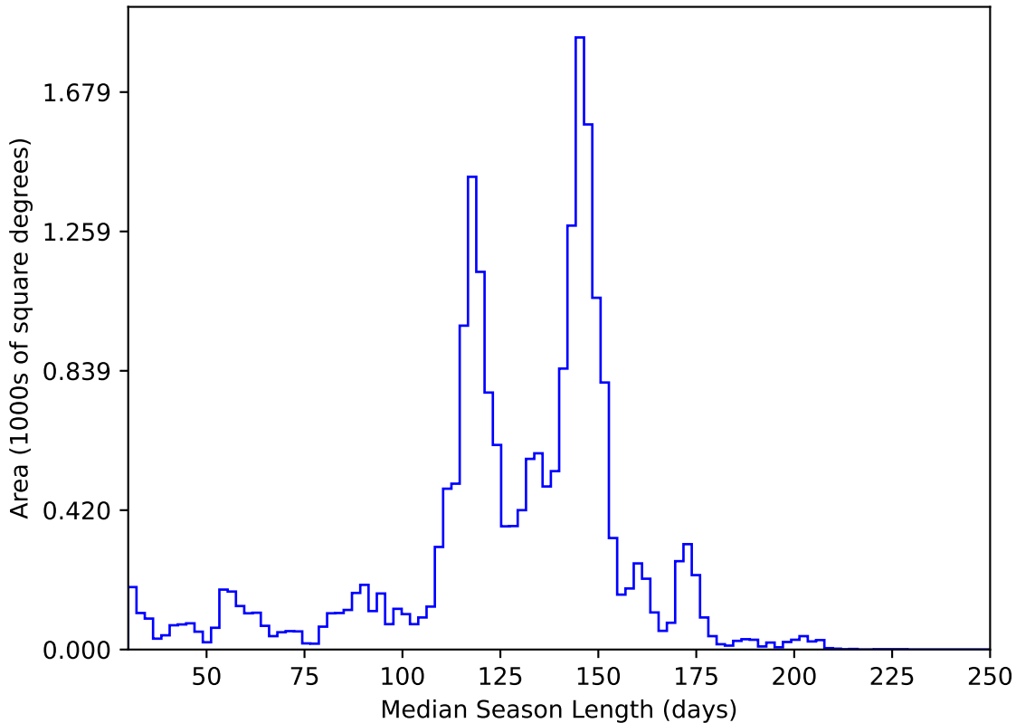
too_elab_r128_d2_gz_v3.4_10yrs All sky y band: Median Season Length
