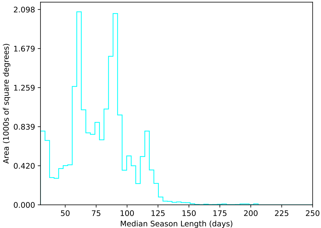
too_elab_r128_d2_gz_v3.4_10yrs All sky u band: Median Season Length
