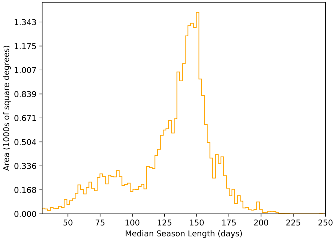
too_elab_r128_d2_gz_v3.4_10yrs All sky r band: Median Season Length
