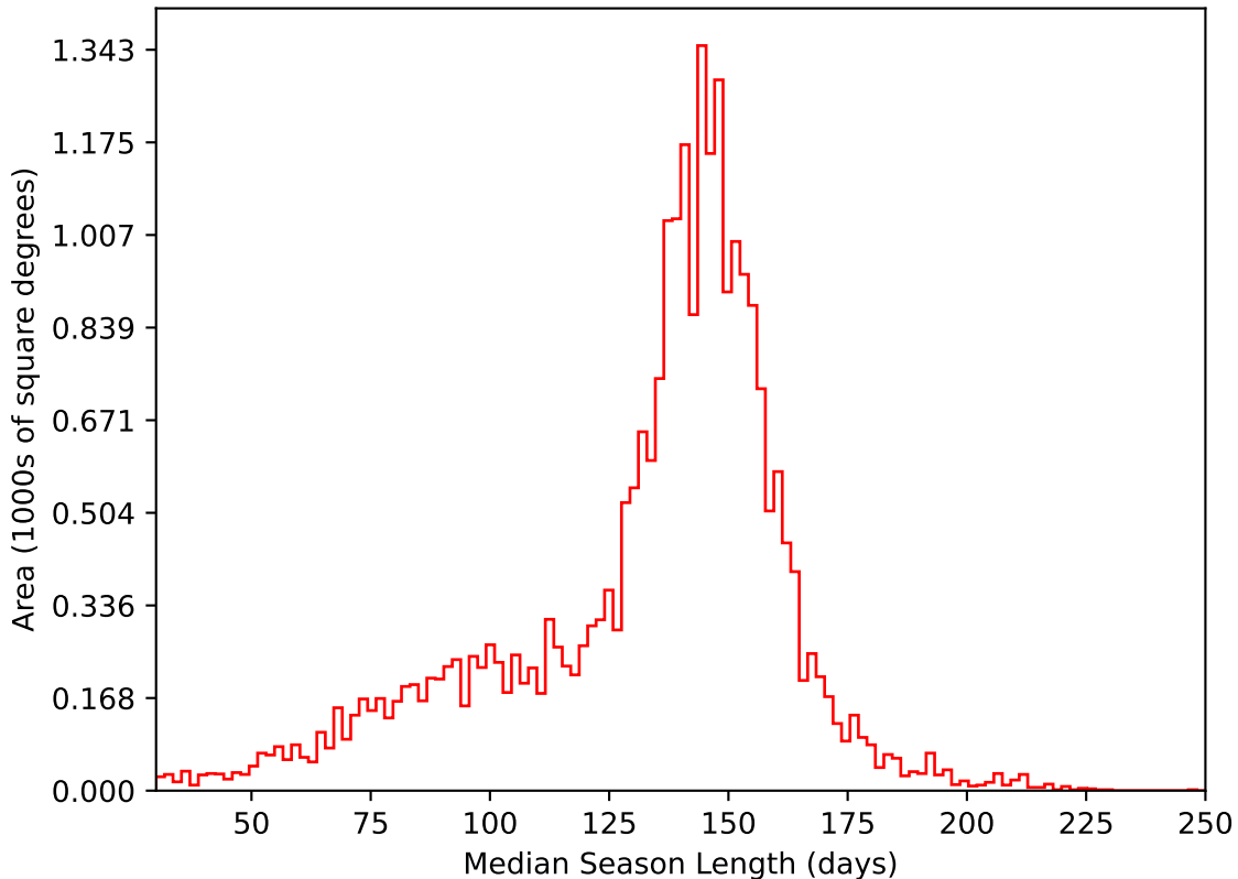
too_elab_r128_d2_gz_v3.4_10yrs All sky i band: Median Season Length
