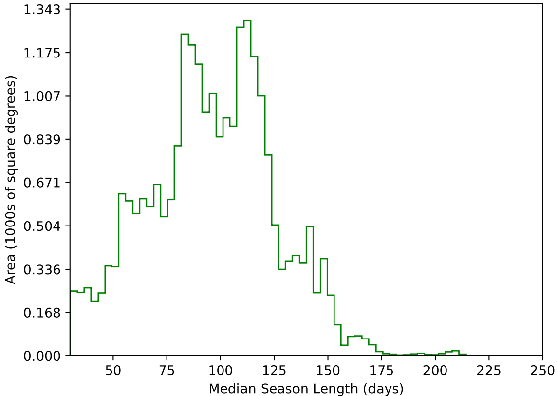
too_elab_r128_d2_gz_v3.4_10yrs All sky g band: Median Season Length
