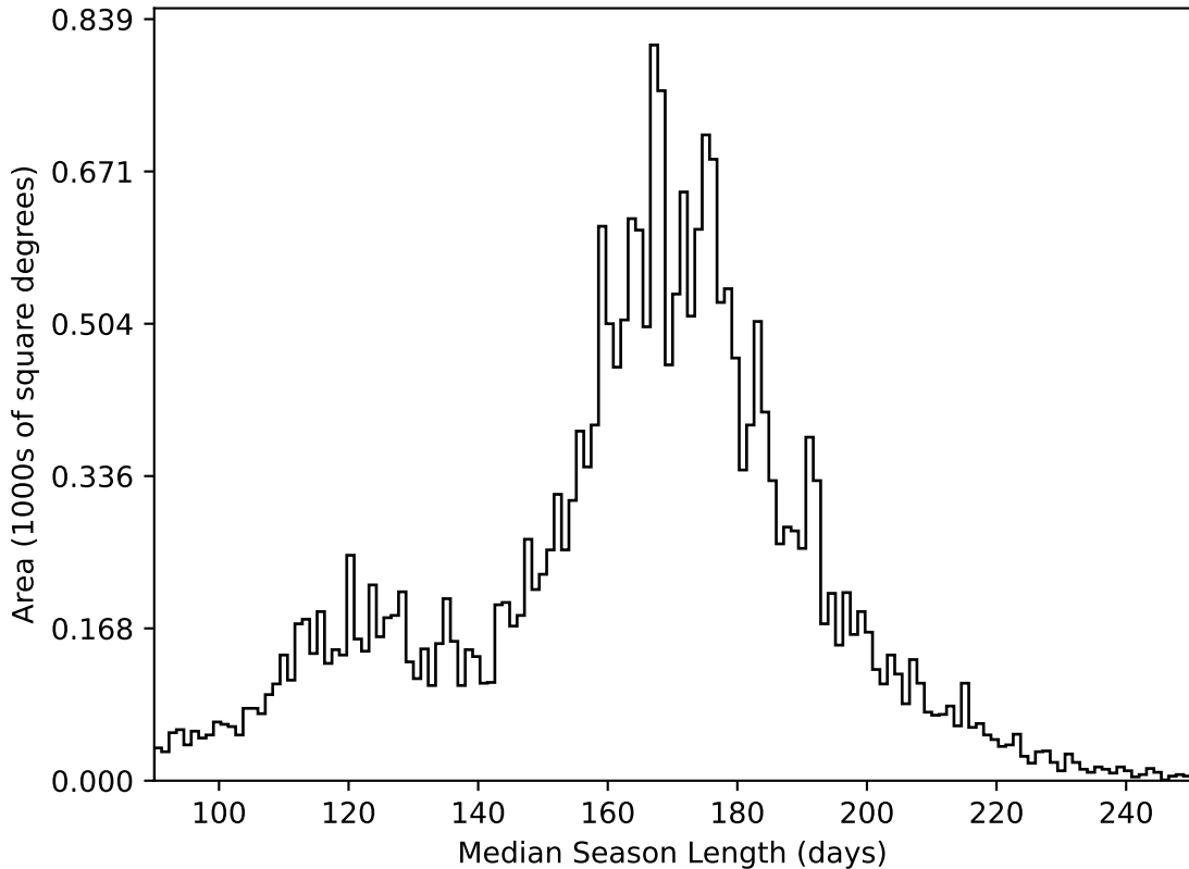
too_elab_r128_d2_gz_v3.4_10yrs All sky all bands: Median Season Length
