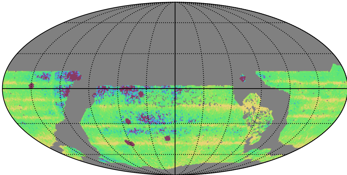
too_elab_r128_d2_gz_v3.4_10yrs WFD: Median Intra-Night Gap
