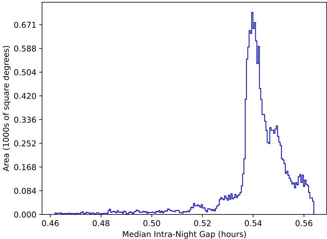
too_elab_r128_d2_gz_v3.4_10yrs WFD: Median Intra-Night Gap
