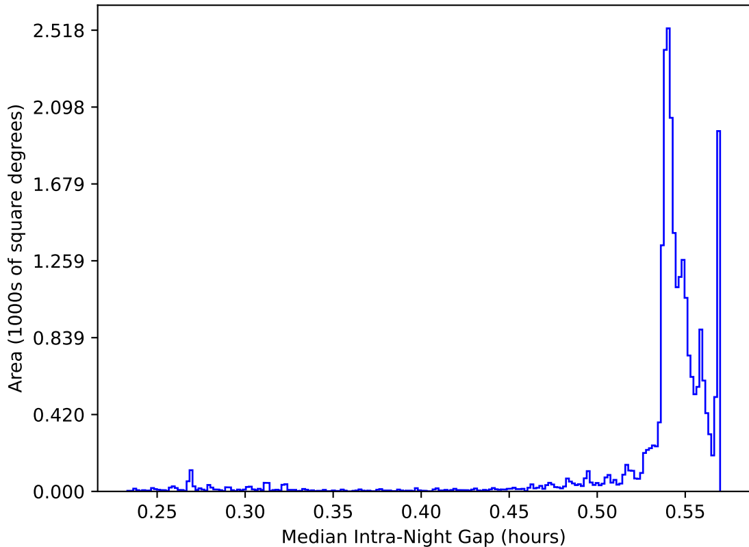
too_elab_r128_d2_gz_v3.4_10yrs All sky: Median Intra-Night Gap
