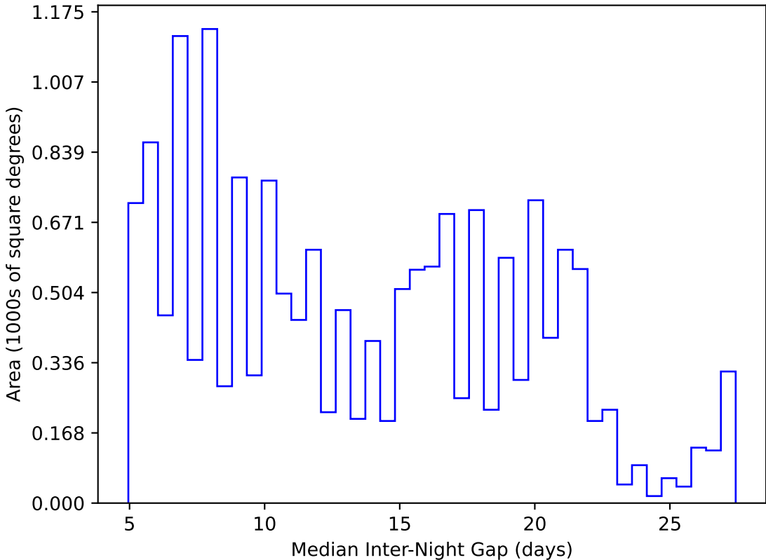
too_elab_r128_d2_gz_v3.4_10yrs WFD y band: Median Inter-Night Gap
