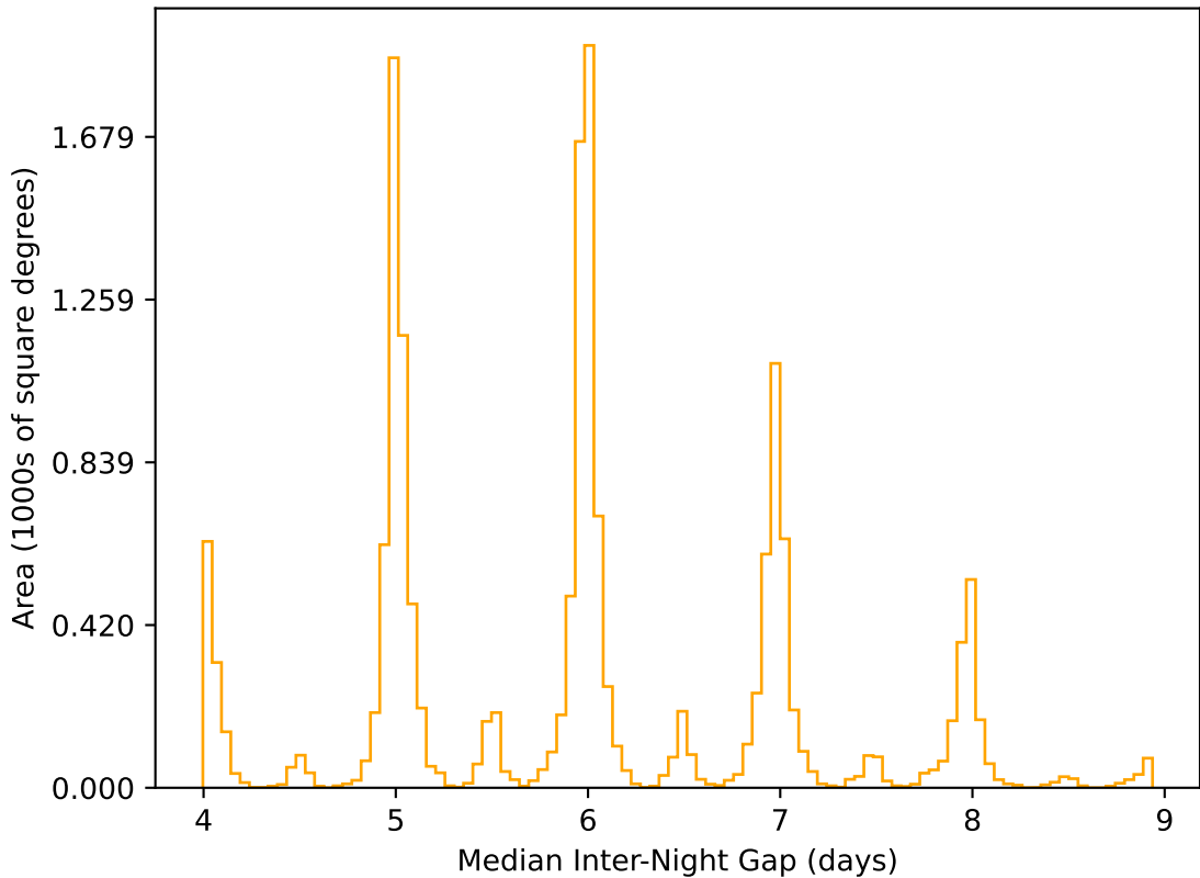
too_elab_r128_d2_gz_v3.4_10yrs WFD r band: Median Inter-Night Gap
