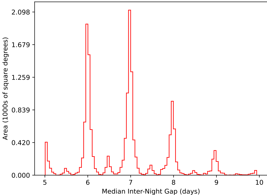
too_elab_r128_d2_gz_v3.4_10yrs WFD i band: Median Inter-Night Gap
