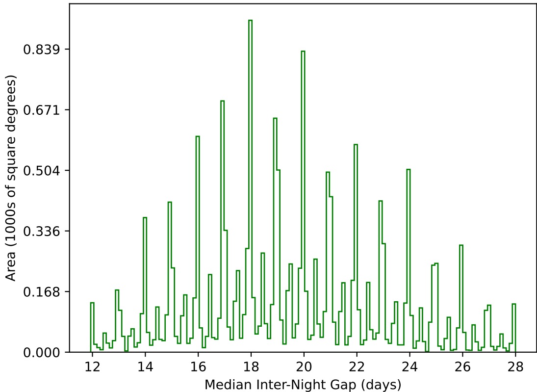
too_elab_r128_d2_gz_v3.4_10yrs WFD g band: Median Inter-Night Gap
