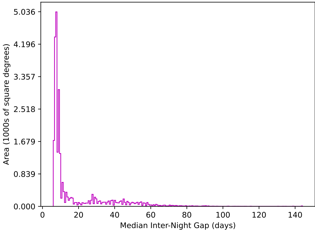
too_elab_r128_d2_gz_v3.4_10yrs All sky z band: Median Inter-Night Gap
