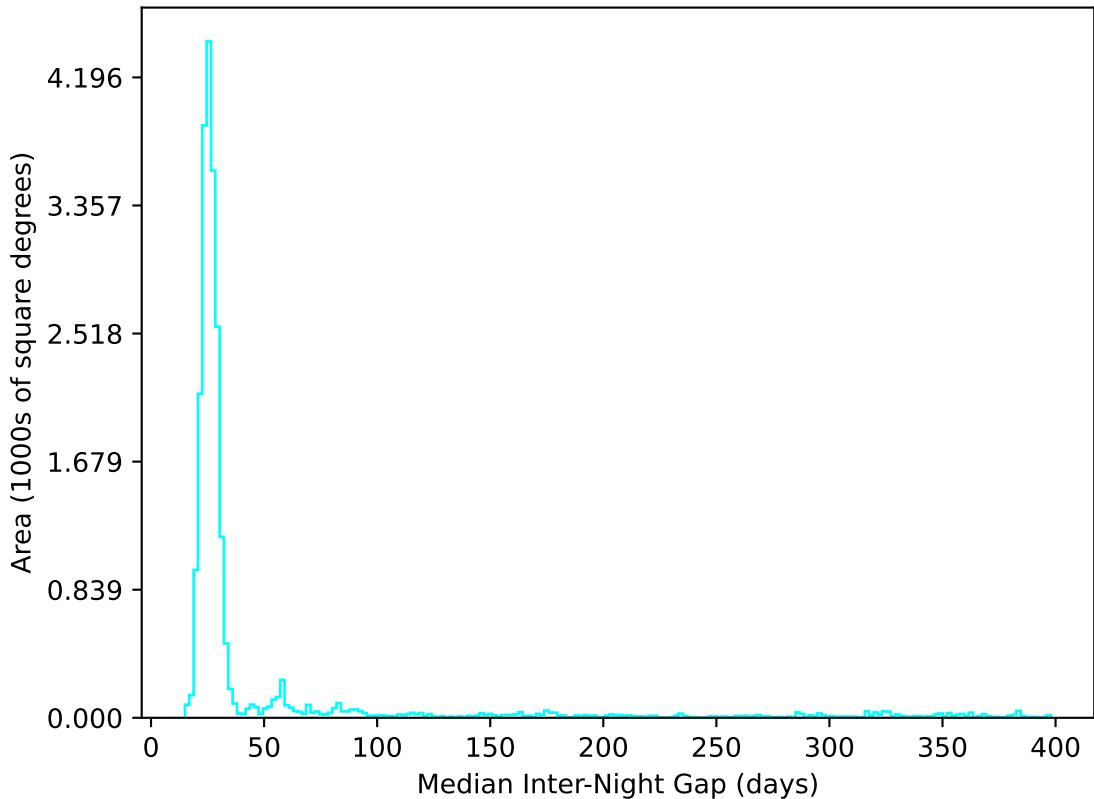
too_elab_r128_d2_gz_v3.4_10yrs All sky u band: Median Inter-Night Gap
