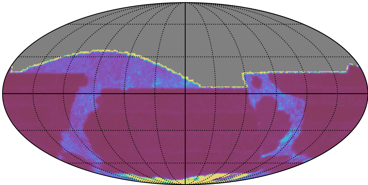
too_elab_r128_d2_gz_v3.4_10yrs All sky r band: Median Inter-Night Gap
