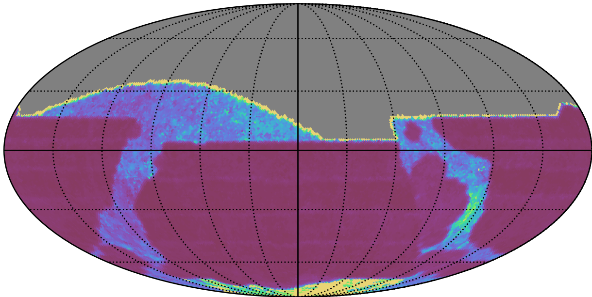
too_elab_r128_d2_gz_v3.4_10yrs All sky i band: Median Inter-Night Gap
