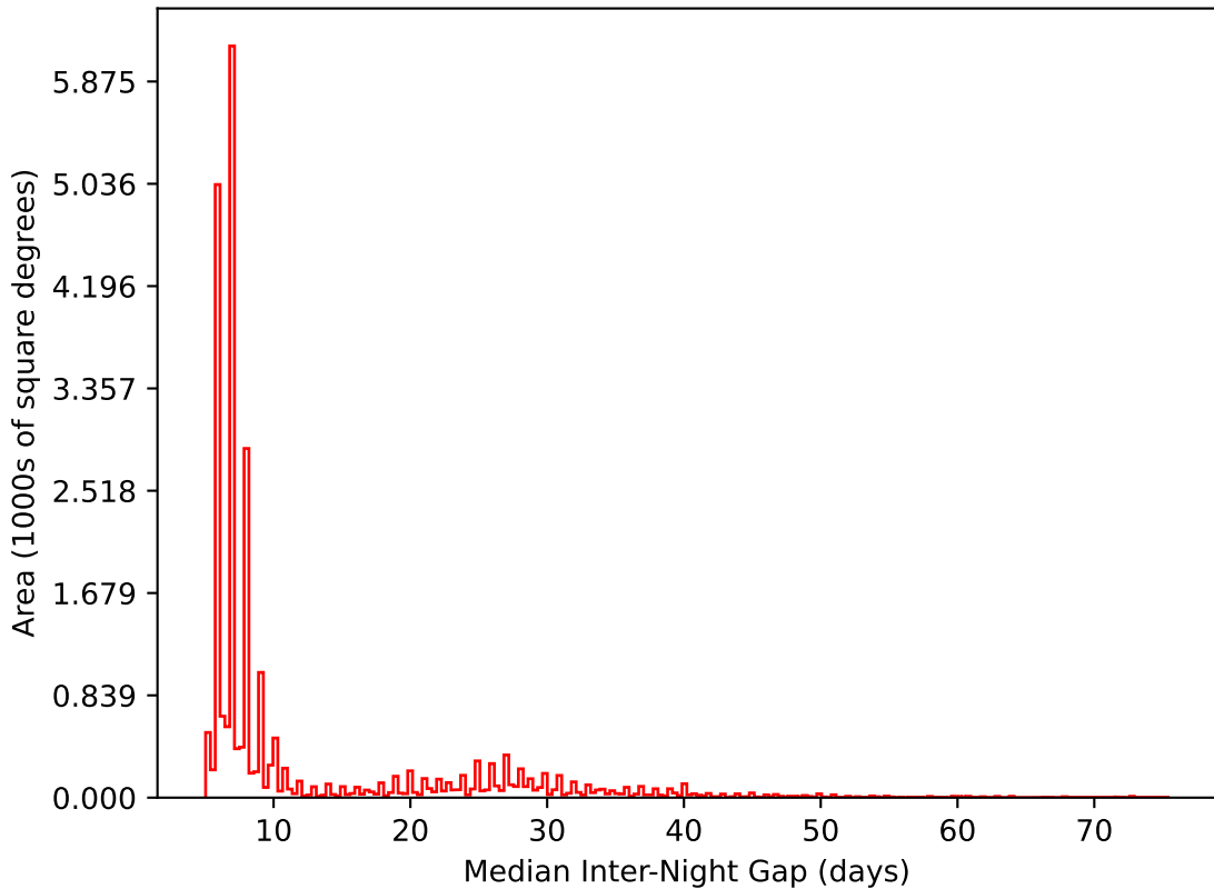
too_elab_r128_d2_gz_v3.4_10yrs All sky i band: Median Inter-Night Gap
