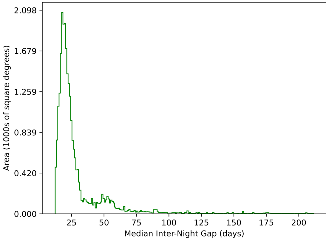
too_elab_r128_d2_gz_v3.4_10yrs All sky g band: Median Inter-Night Gap
