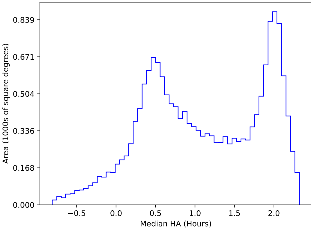
too_elab_r128_d2_gz_v3.4_10yrs WFD z band: Median HA
