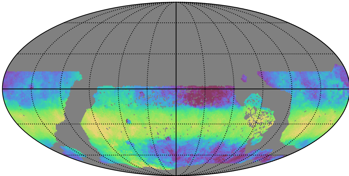
too_elab_r128_d2_gz_v3.4_10yrs WFD y band: Median HA
