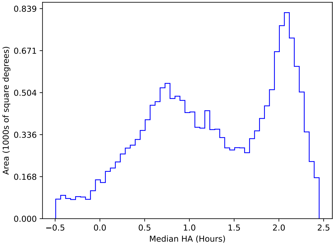
too_elab_r128_d2_gz_v3.4_10yrs WFD y band: Median HA
